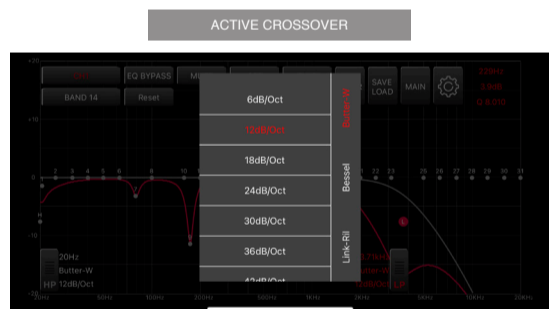
Active crossover allows HPF (high pass filter), LPF (low pass filter) and BPF (band pass filter) with the full 20Hz-20Khz available to all bands. The crossover slope is also variable between 6dB and 48dB Octaves.
